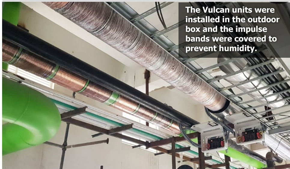
S250 for the extruder chilled water line
