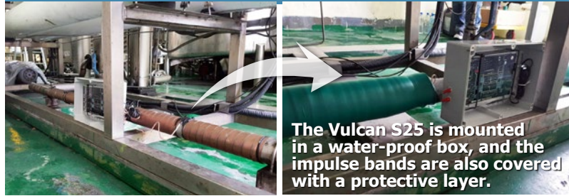
Vulcan S25 installed on the 4" circulating water pipe
